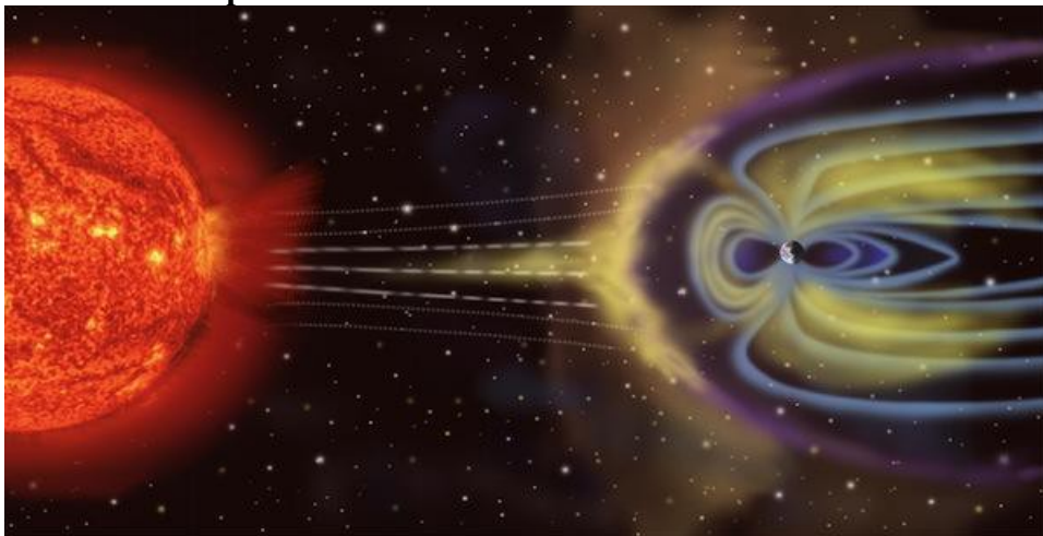
Image 2. The Sun hits Earth's protective magnetic field with a CME (coronal mass ejection), and/or a solar flare; artist's rendition[76]
