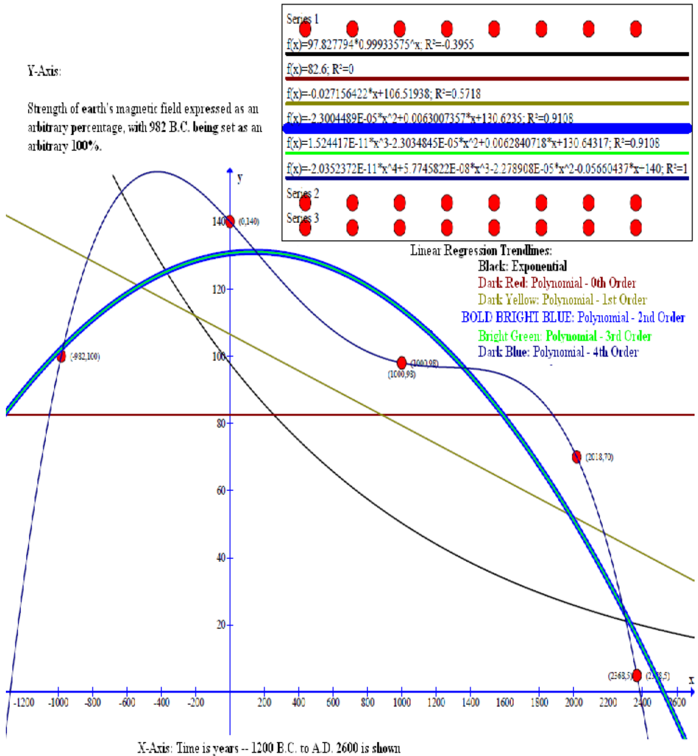
Image 10. “Linear Regression” GRAPH of changes in the dipole strength of Earth's protective geomagnetic field, as a function of time. DATA used for this graph are the five (5) data points taken from Table 4. of this paper, and using “5%” for the 5 th and last data point, where a choice is given.
