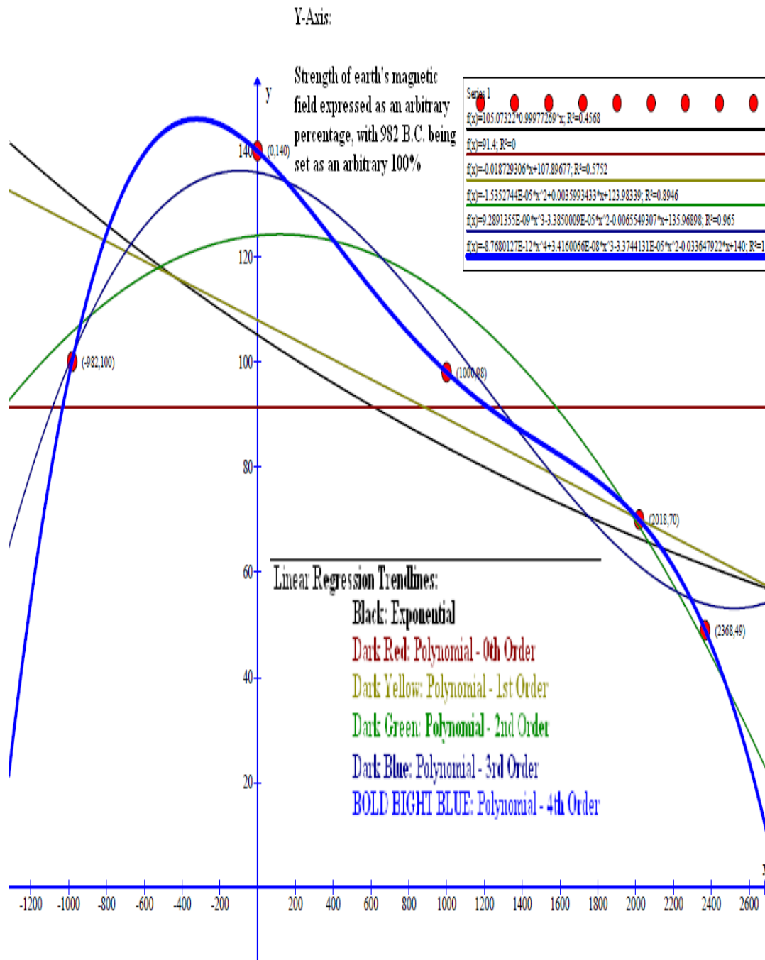
Image 9. "Linear Regression" GRAPH of changes in the dipole strength of earth's protective geomagnetic field, as a function of time. DATA used for this graph are the five (5) data points taken from Table 4. of this paper, and using "49%" for the 5th and last data point, where a choice is given.
