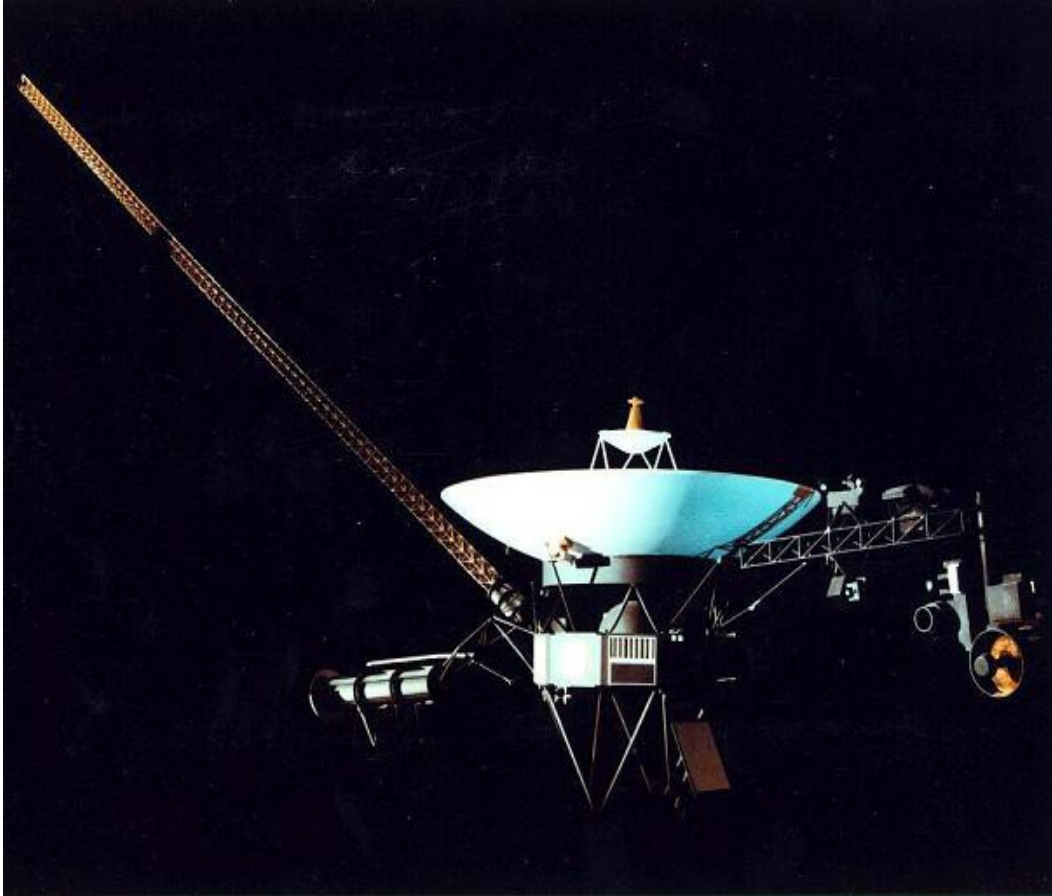
Image 8. Photo of one of the Voyager spacecraft, of NASA's “deep space” Mariner series, and a reminder that similar satellites and NASA equipment, closer to Earth, are vulnerable to solar geomagnetic events[82]
