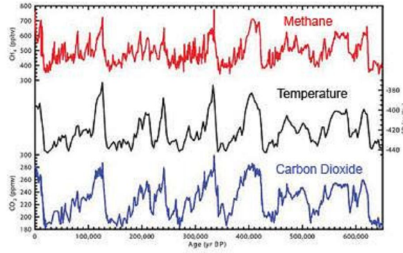
Figure 3. Comparison of carbon dioxide and temperature in ice cores. 7
